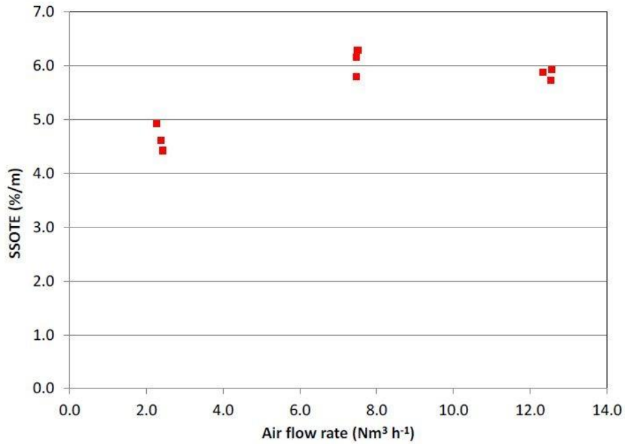
Specific standard oxygen transfer efficiency against air flow rate (Aquaflex tube diffuser ATD63-1000 - 5.8 m of submergence)
